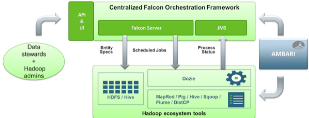
Figure 3.1. Falcon Architecture
