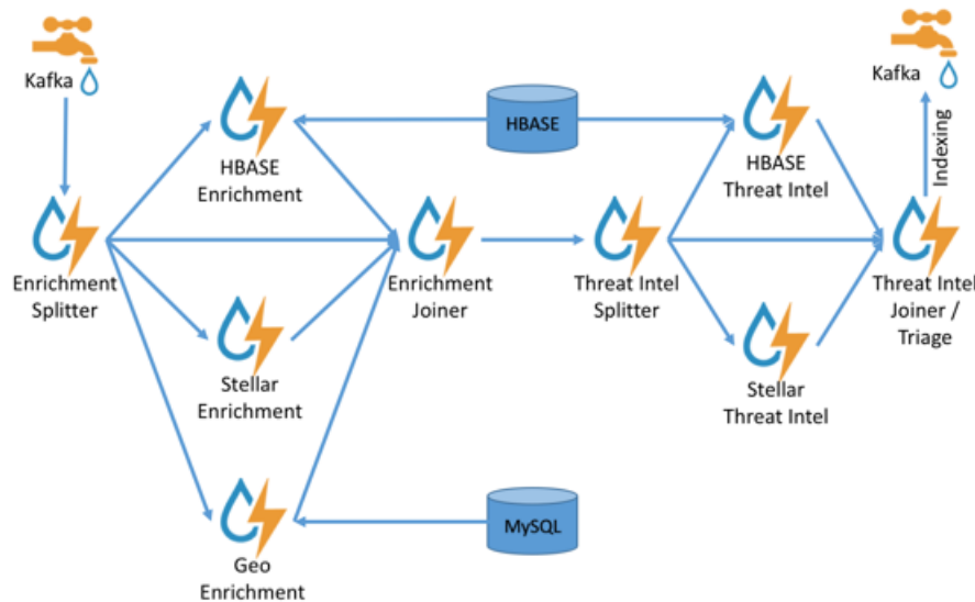
HCP Enrichment Flow
